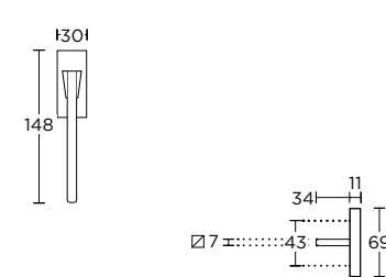
TILT & TURN WINDOW HANDLE
