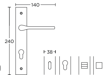
HANDLE ON PLATE
